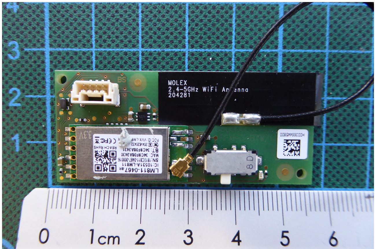
181920_7: BT/WLAN-module, top view
