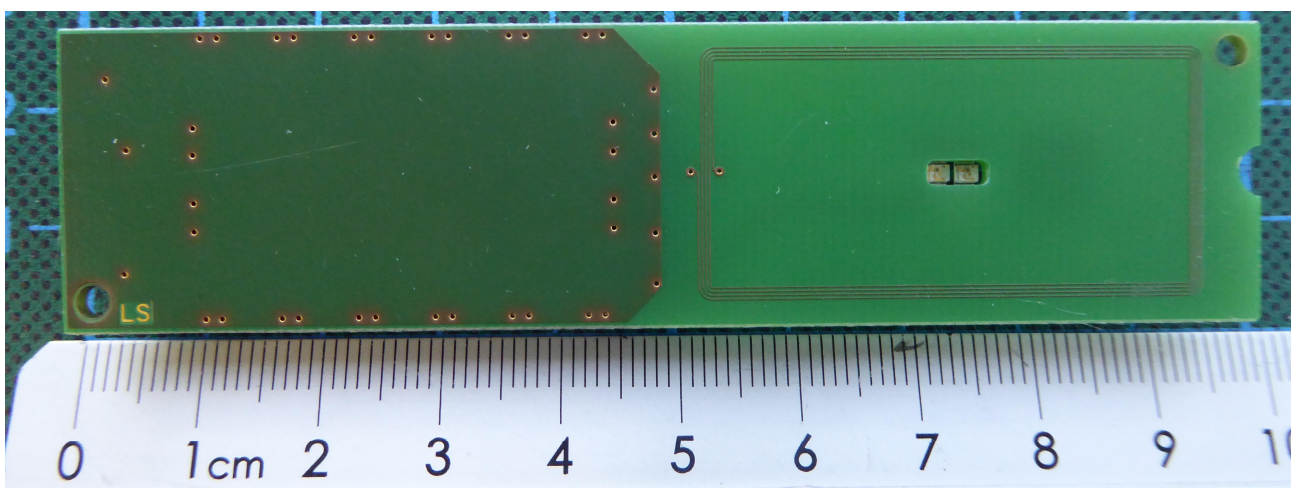
181920_6: NFC/RFID-module, bottom view
